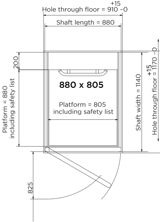
Platform 880 x 805
